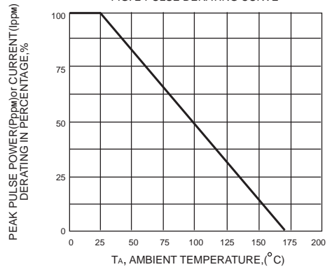
FIG. 2-PULSE DERATING CURVE
