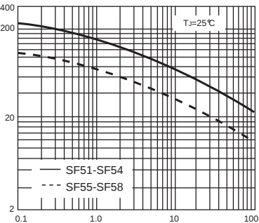
FIG. 5-TYPICAL JUNCTION CAPACITANCE
