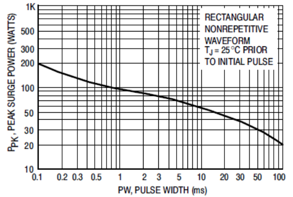
Figure 3. Maximum Surge Power
