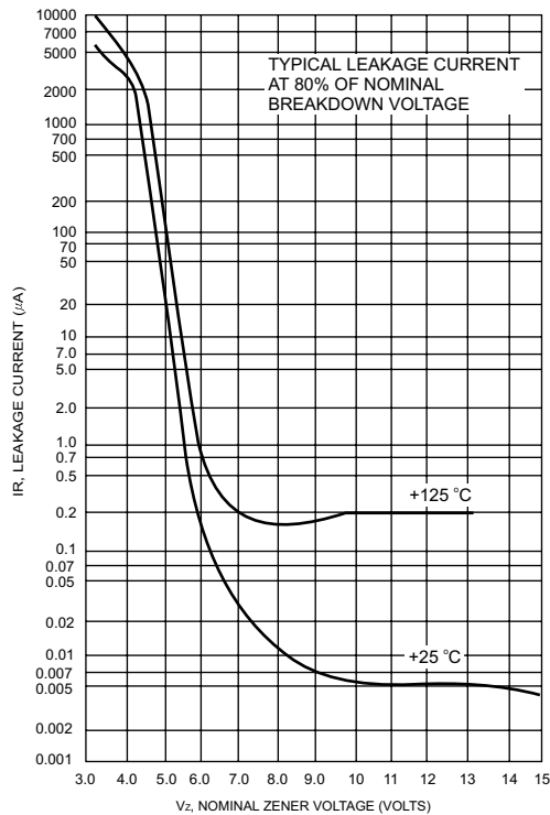
FIG.2- TYPICAL LEAKAGE CURRENT
