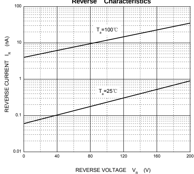
Reverse Characteristics
