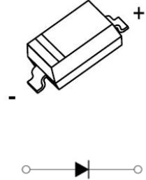
SOD-123
