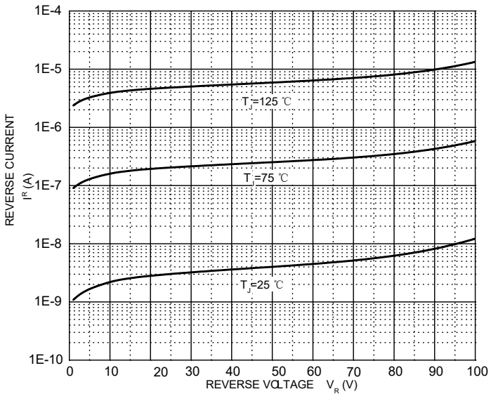
Reverse Characteristics
