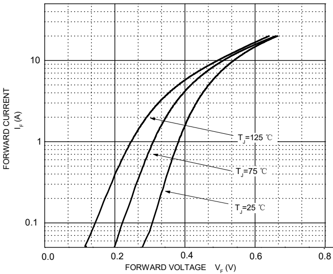
Forward Characteristics
