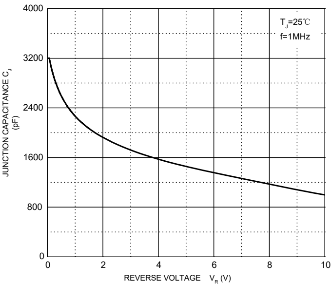
Capacitance Characteristics Per Diode
