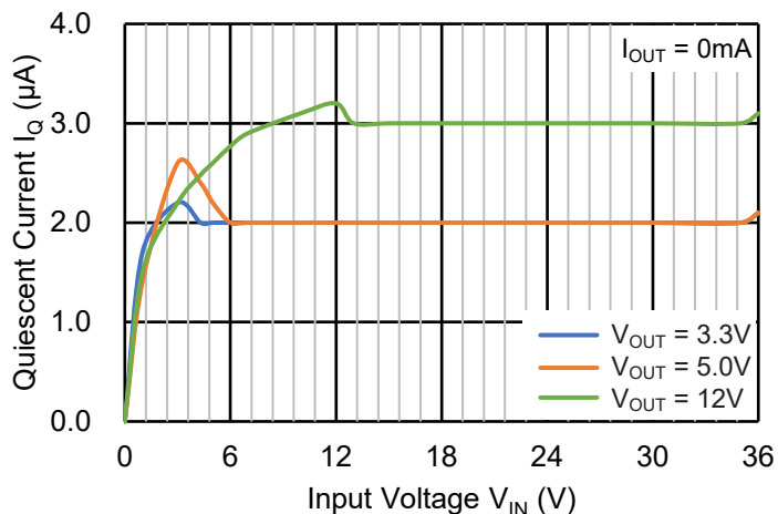
Quiescent Current
