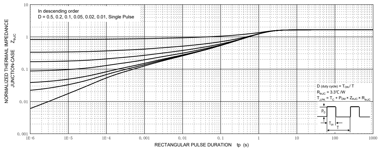
MURF20H60L Transient Thermal Impedance, Junction-Case
