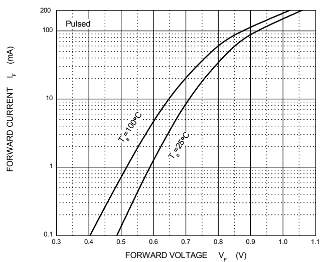
Forward Characteristics
