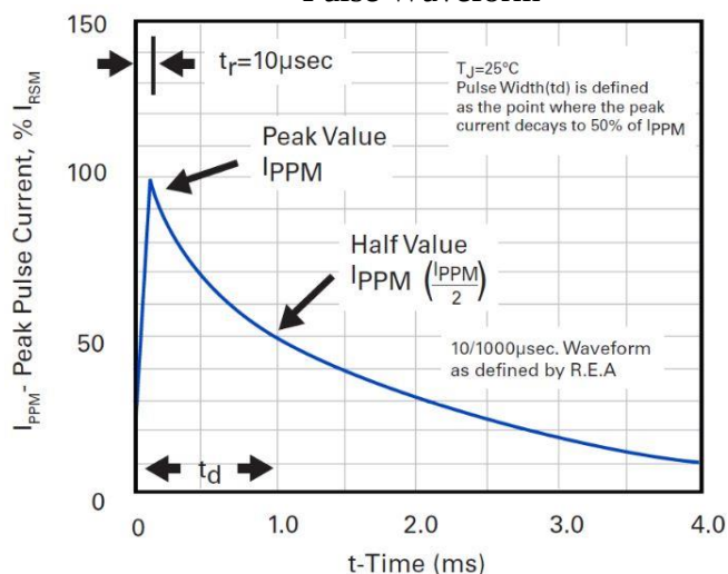
Pulse Waveform
