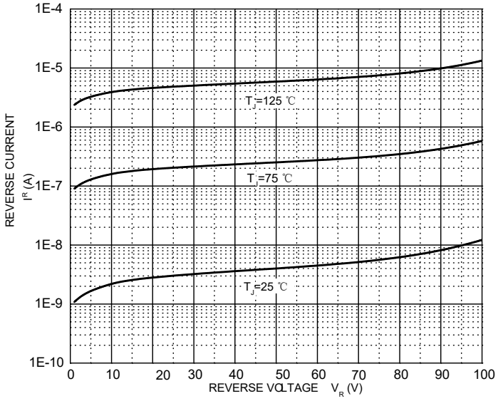
Reverse Characteristics
