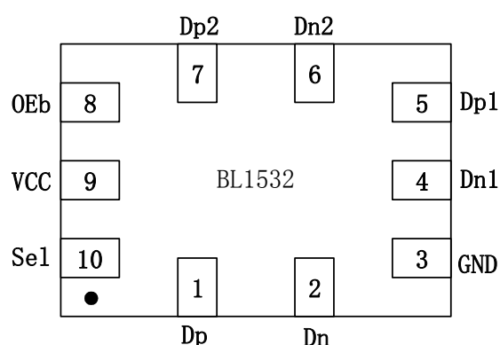
UTQFN1.8×1.4-10L
