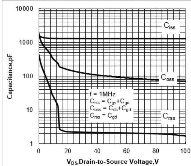
Figure 10 Capacitance Characteristics
