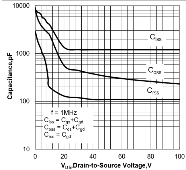
Figure 10 Capacitance Characteristics
