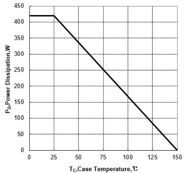
Figure 2 Power Dissipation
