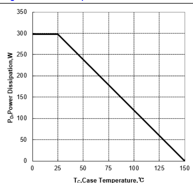
Figure 2 Power Dissipation
