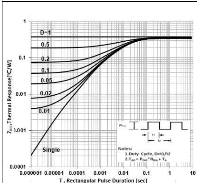
Figure 3 Max Thermal Impedance (No FullPAK)
