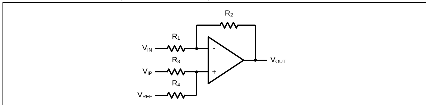
Figure 1. Differential Amplifier
