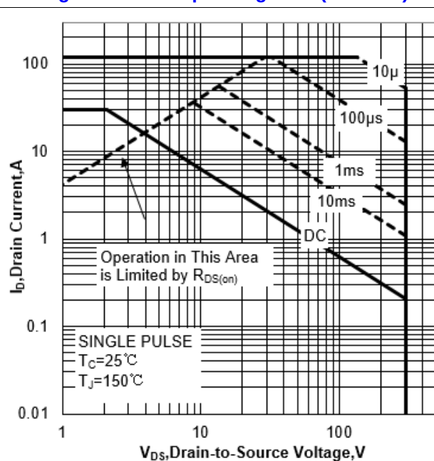
Figure 1b Safe Operating Area (TO-220F)
