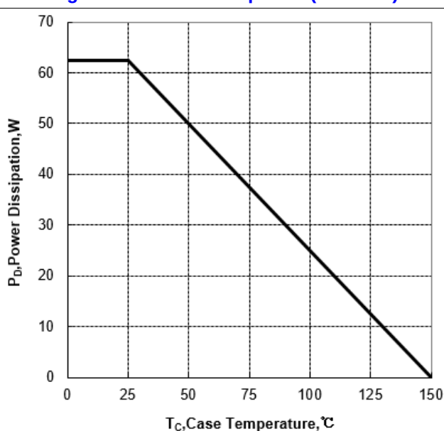
Figure 2b Power Dissipation (TO-220F)
