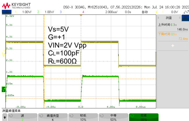
Slew Rate
