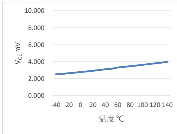
V_{OL} vs. Temperature
