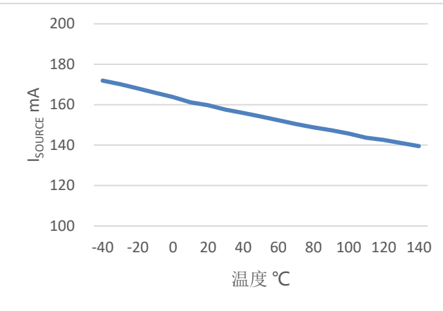
I_{SOURCE} vs. Temperature
