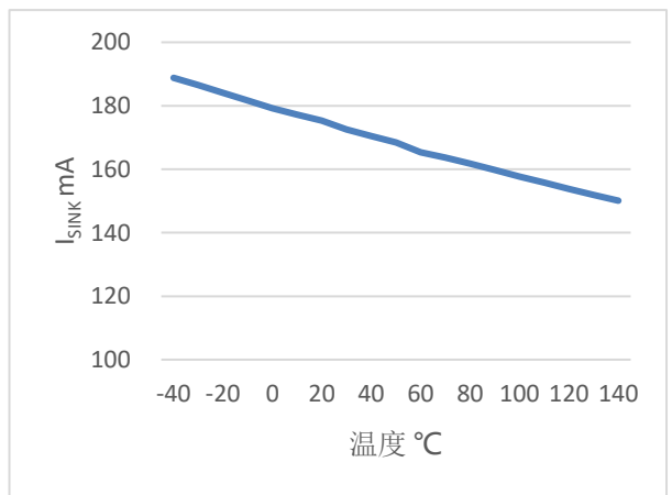
I_{SINK} vs. Temperature
