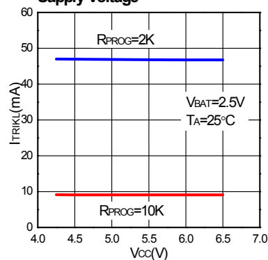
Trickle Charge Current vs Supply Voltage
