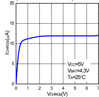
CHRGb Pin I-V Curve (Weak Pull-Down State)
