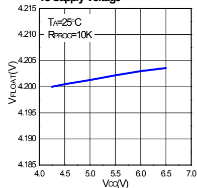
Regulated Output (Float) Voltage vs Supply Voltage
