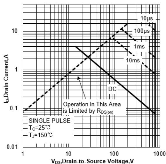
Figure 1b Safe Operating Area (FullPAK)
