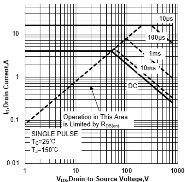
Figure 1a Safe Operating Area (No FullPAK)
