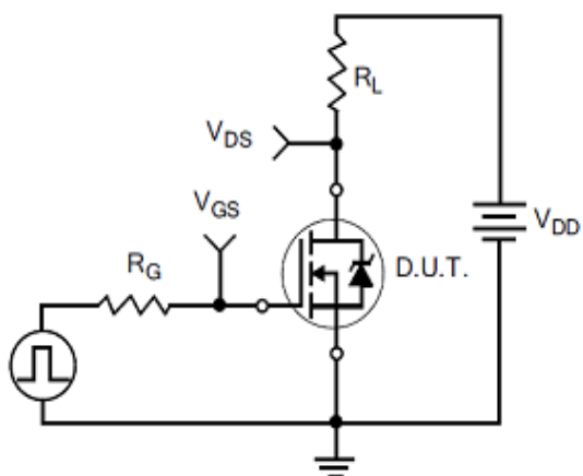
Figure 14 Resistive Switching Test Circuit
