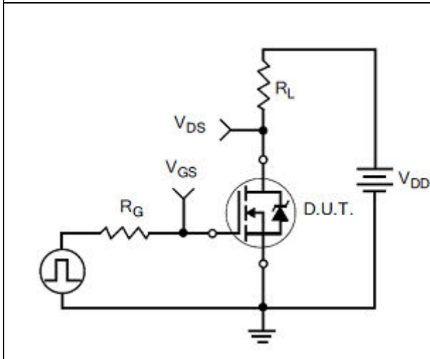
Figure 14 Resistive Switching Test Circuit
