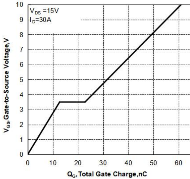
Figure 7 Gate-Charge Characteristics
