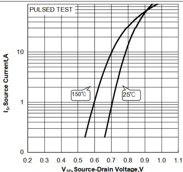
Figure 9 Body Diode Forward Voltage
