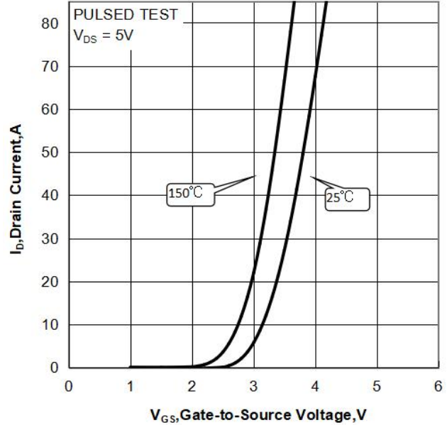
Figure 2 Transfer Characteristics
