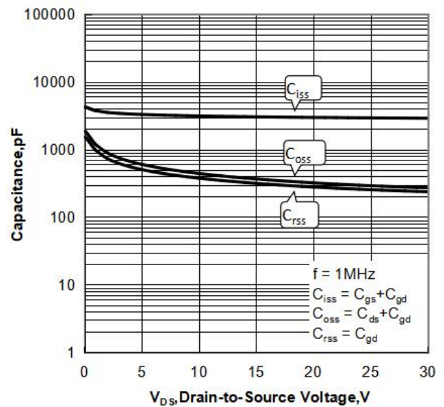
Figure 8 Capacitance Characteristics
