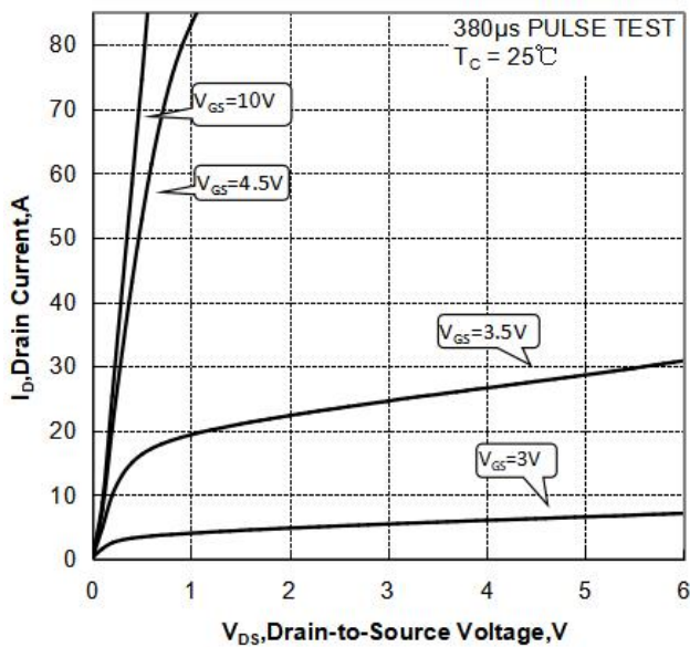
Figure 1 Output Characteristics
