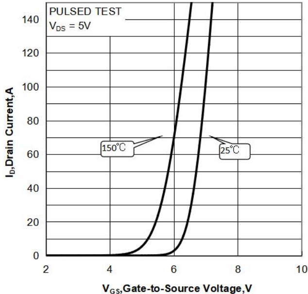
Figure 2 Transfer Characteristics
