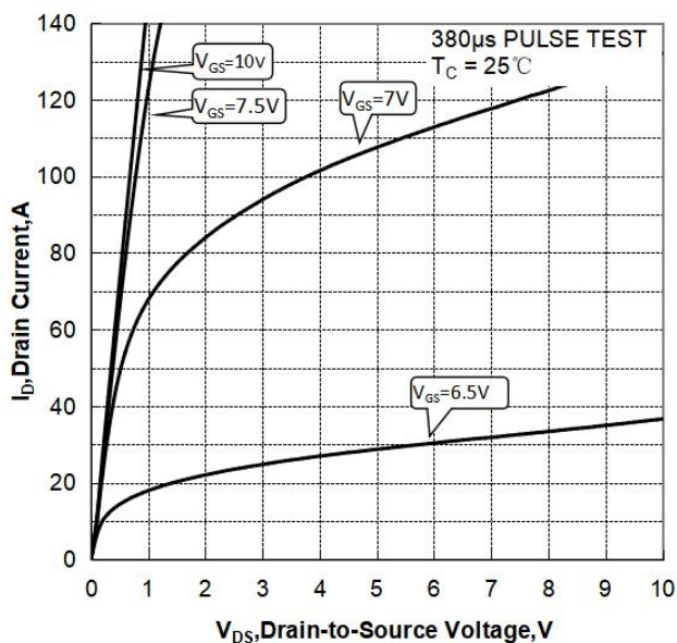
Figure 1 Output Characteristics
