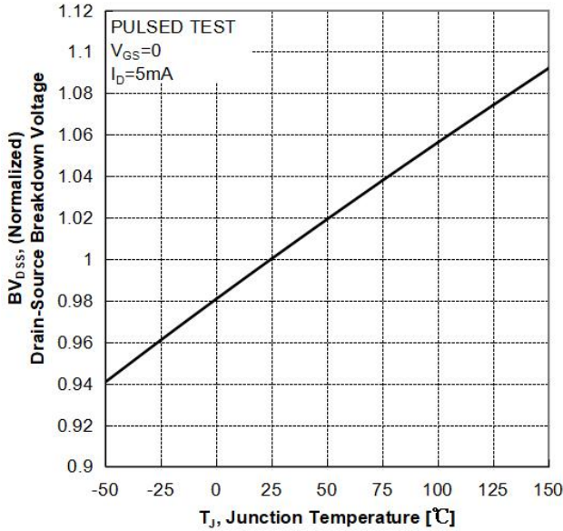
Figure 5 BV vs Junction Temperature
