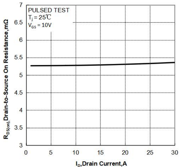
Figure 3 On-Resistance vs. I_D
