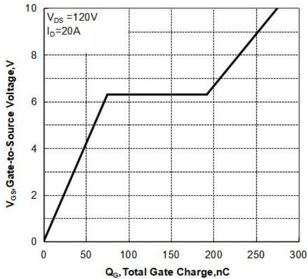
Figure 7 Gate-Charge Characteristics
