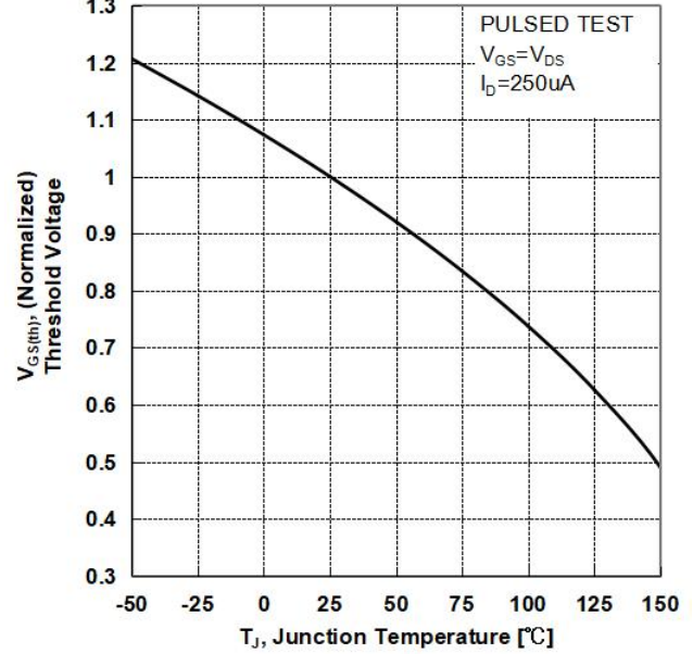
Figure 6 Vth vs Junction Temperature
