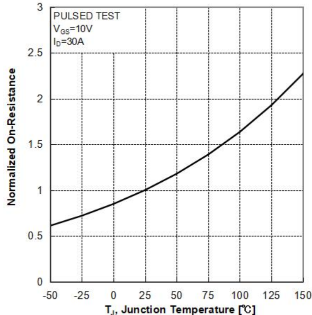
Figure 4 On-Resistance vs. Junction Temperature
