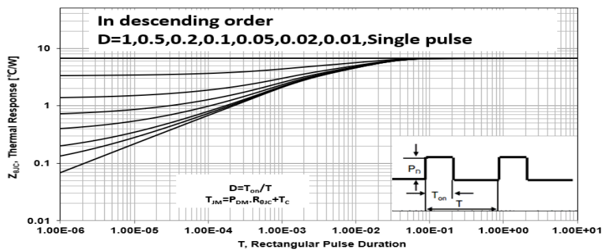
Figure 11 Transient Thermal Impedance
