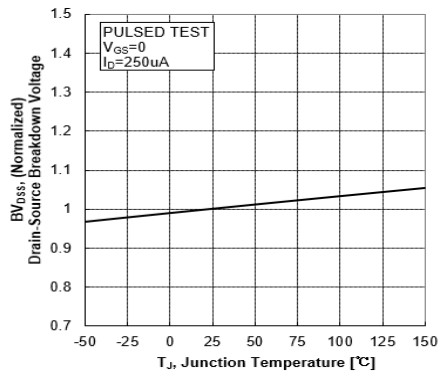
Figure 5 BV vs Junction Temperature
