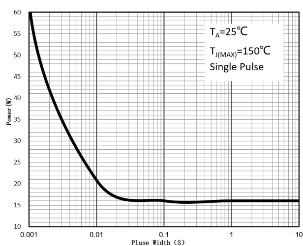
Figure 10a Single Pulse Power Rating Junction-to-Ambient (PDFN3.3*3.3)
