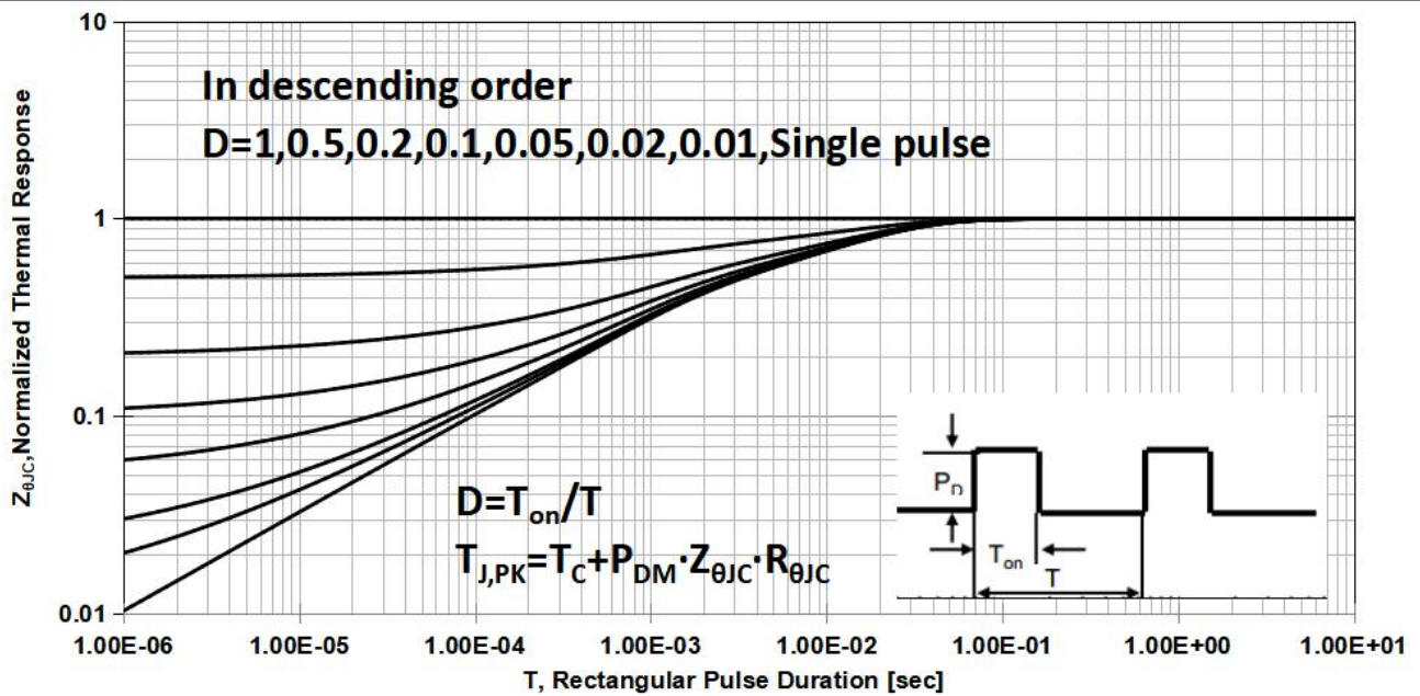
Figure 11a Transient Thermal Impedance (TO-252)
