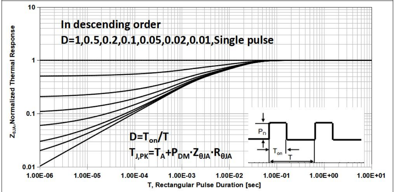
Figure 11d Transient Thermal Impedance (SOP-8)
