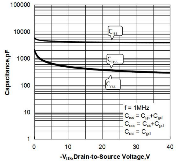
Figure 8 Capacitance Characteristics
