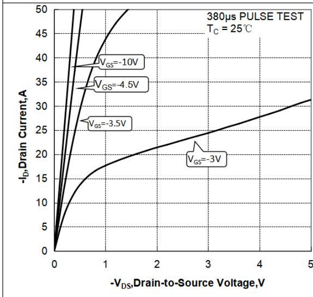
Figure 1 Output Characteristics
