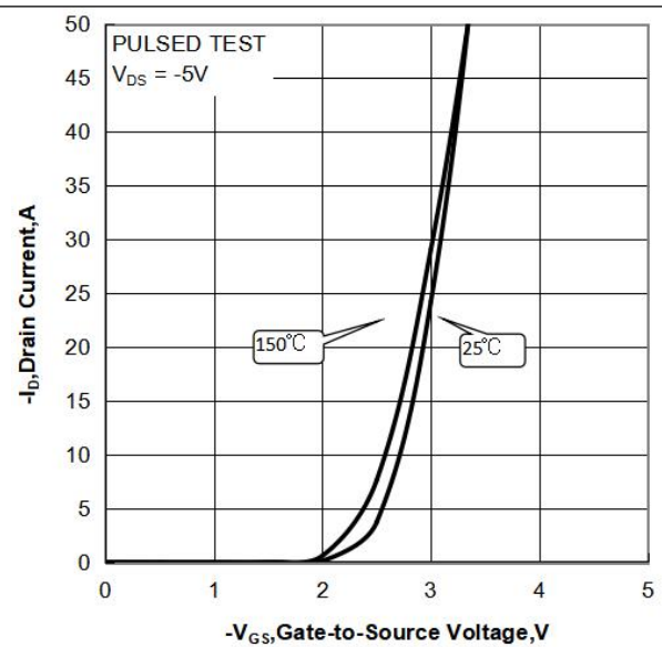
Figure 2 Transfer Characteristics
