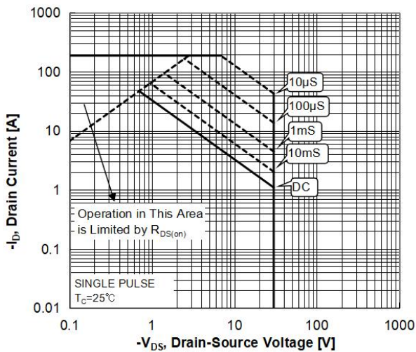
Figure 10b Maximum Safe Operating Area (PDFN5*6)
