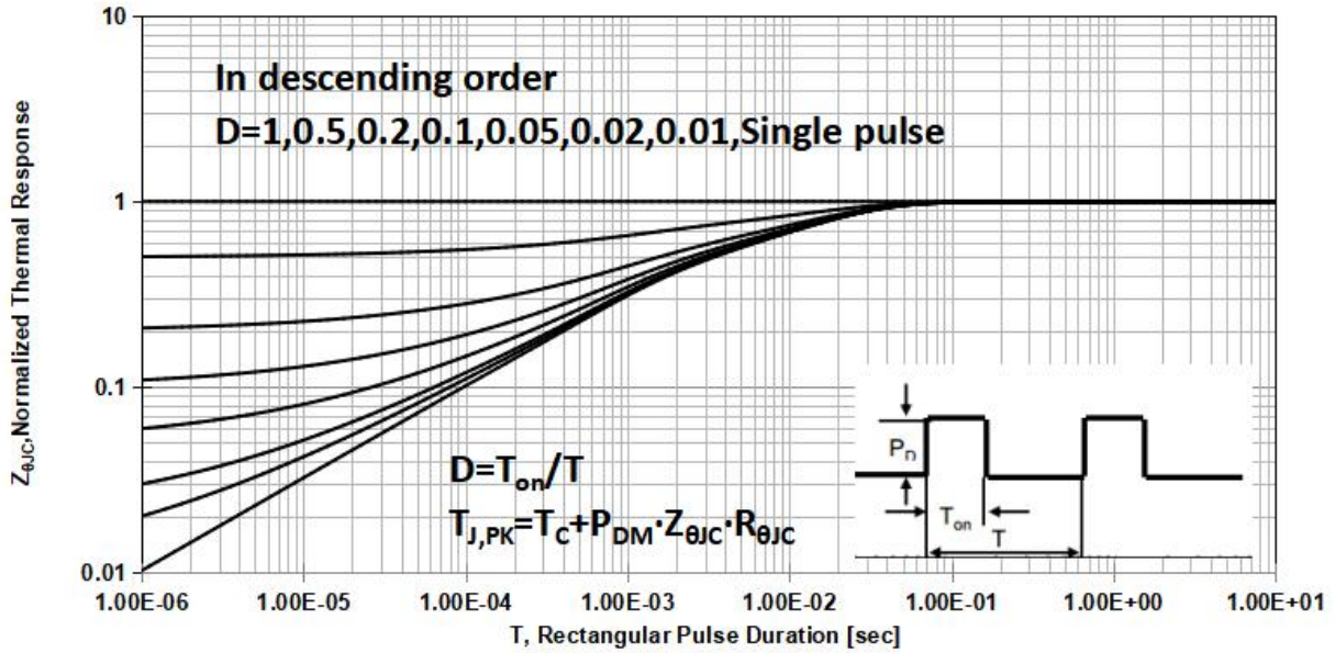
Figure 11b Transient Thermal Impedance(PDFN5*6)
