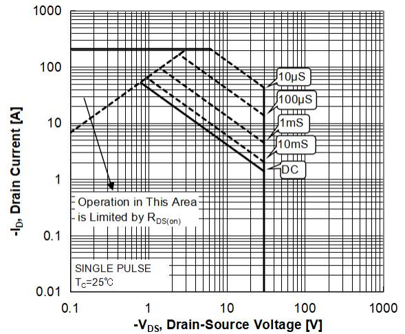
Figure 10a Maximum Safe Operating Area (TO-252)
