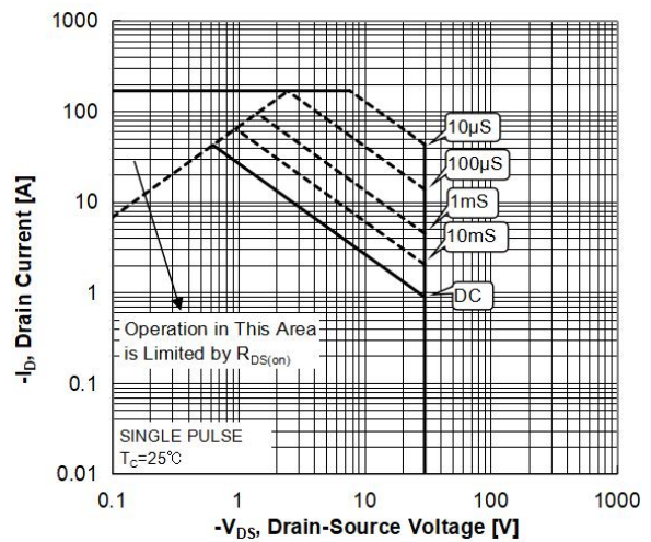
Figure 10c Maximum Safe Operating Area (PDFN3.3*3.3)
