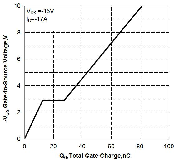
Figure 7 Gate-Charge Characteristics
