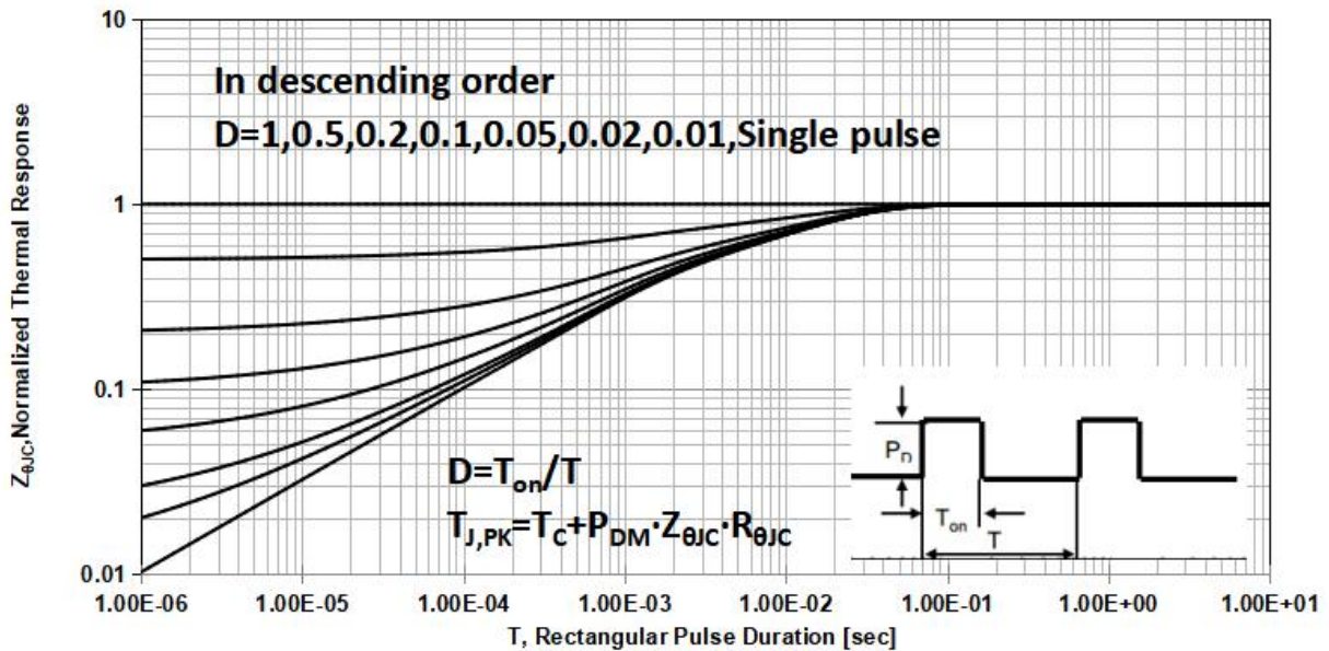
Figure 11c Transient Thermal Impedance(PDFN3.3*3.3)
