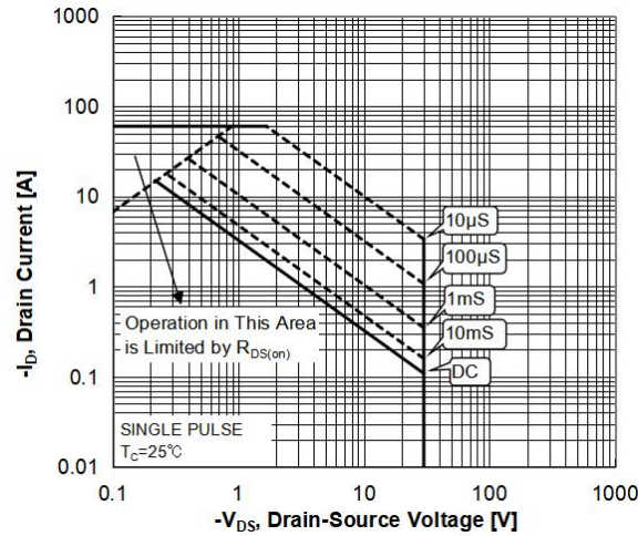
Figure 10d Maximum Safe Operating Area (SOP-8)
