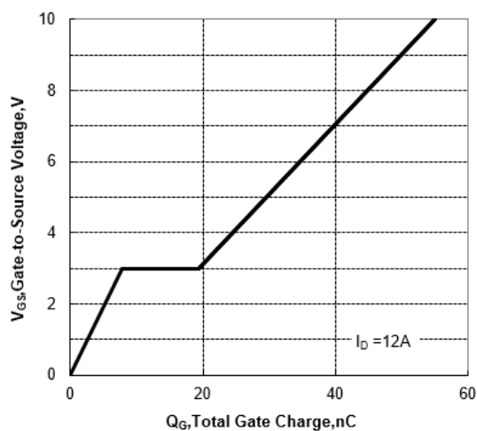
Figure 7 Gate-Charge Characteristics
