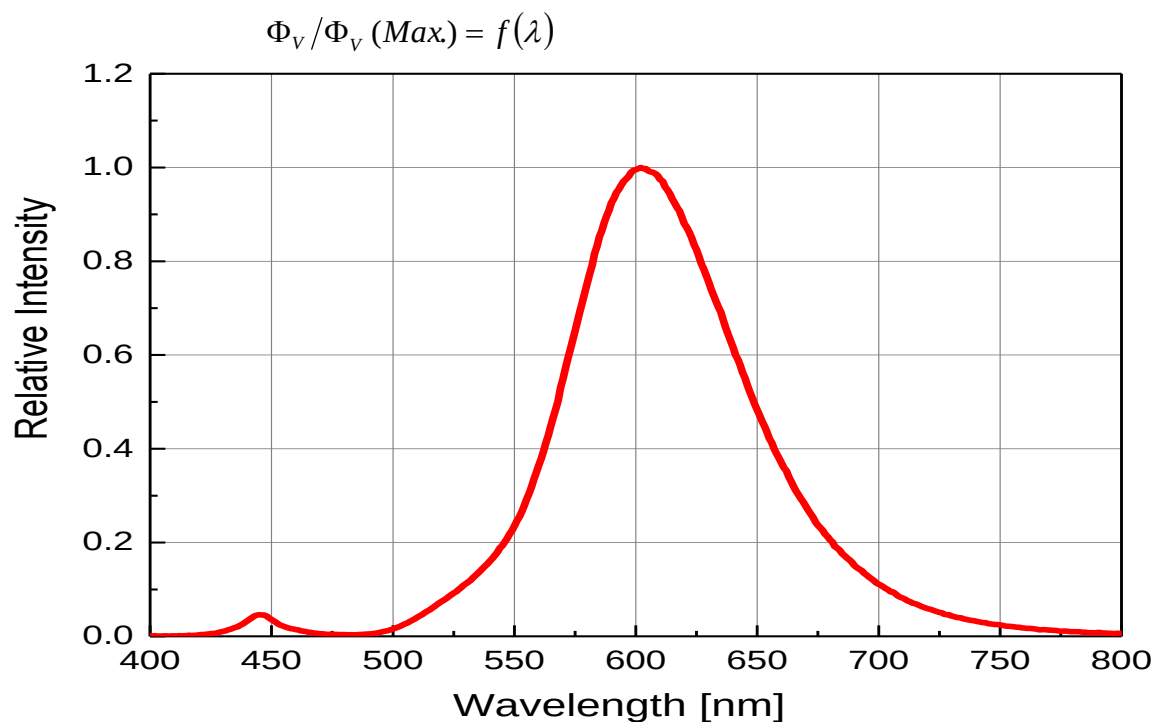
Typical Diagram Characteristics of Radiation
