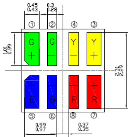
BOT. view
