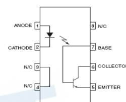
Pin Configuration
