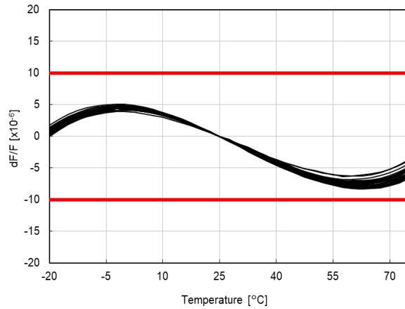
20 MHz n = 30
