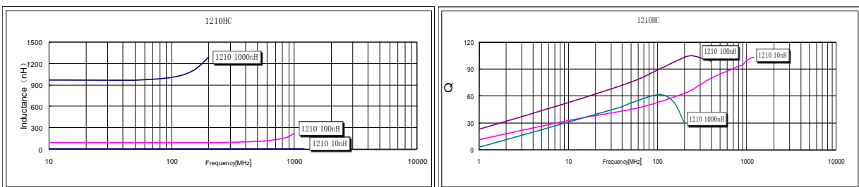
FHW1210 Type.
