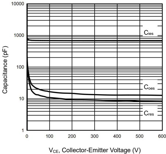
Figure 5 Capacitance Characteristics
