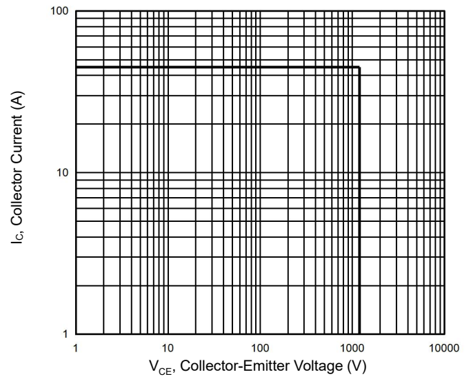
Figure 14 Reverse Bias SOA
