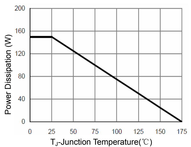
Figure 10 Power De-rating
