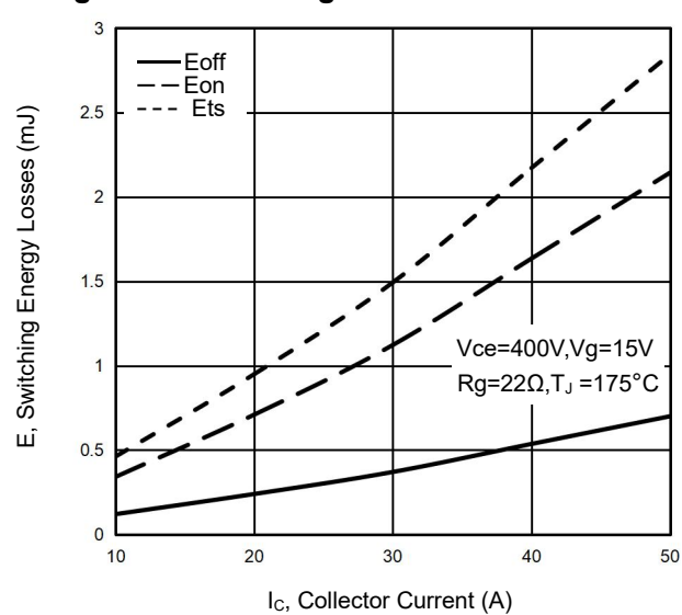
Figure 14 Switching Loss vs. Collector Current
