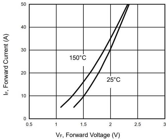
Figure 7 Forward Characteristics
