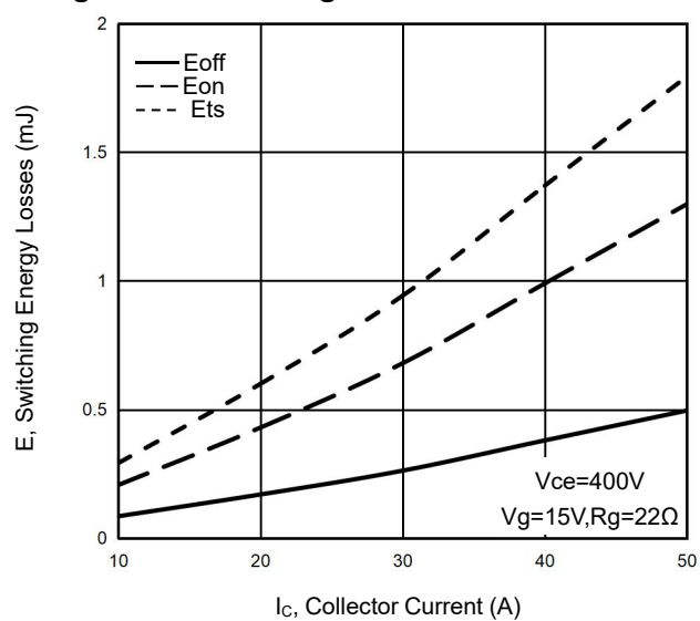
Figure 13 Switching Loss vs. Collector Current
