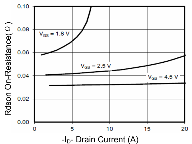
Figure 6 Drain-Source On-Resistance
