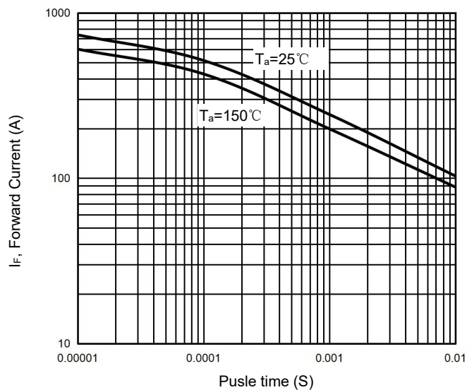
Figure 20 Non-repetitive peak surge forward current versus pulse duration (sinusoidal waveform)
