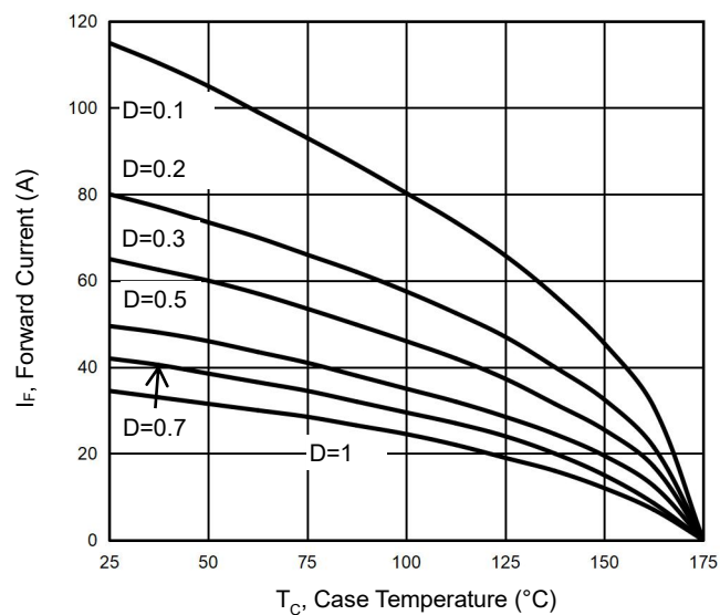
Figure 19 Peak forward current versus case temperature
