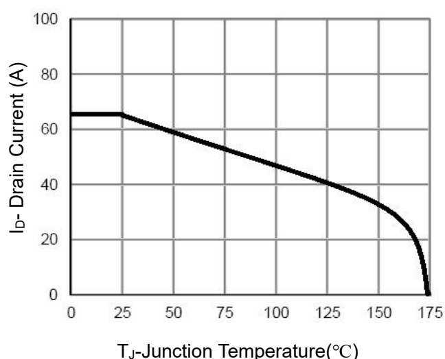
Figure 10 ID Current- Junction Temperature
