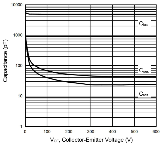
Figure 5 Capacitance Characteristics
