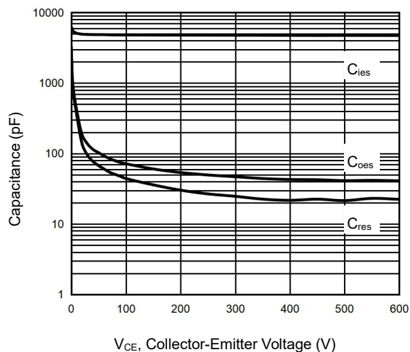
Figure 5 Capacitance Characteristics
