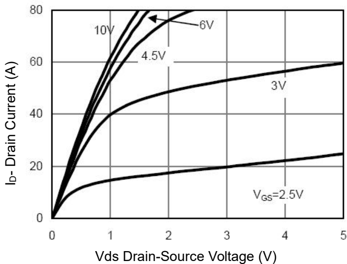
Figure 3 Output Characteristics
