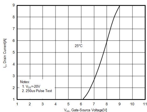
Figure4. Transfer characteristics
