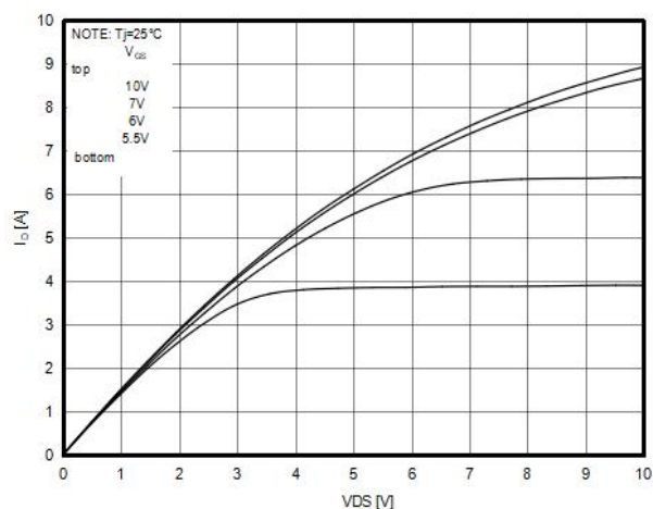
Figure4. Output characteristics
