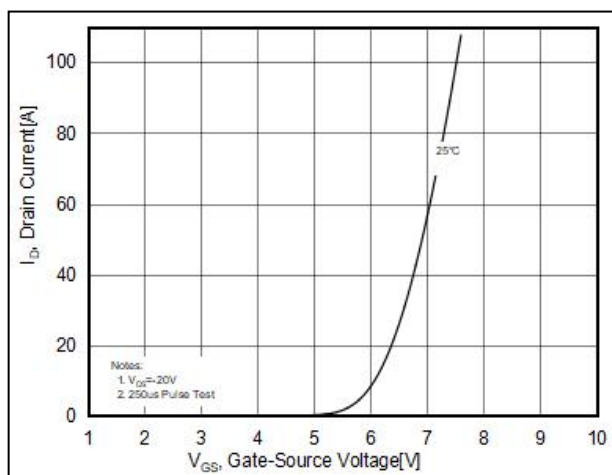
Figure5. Transfer characteristics
