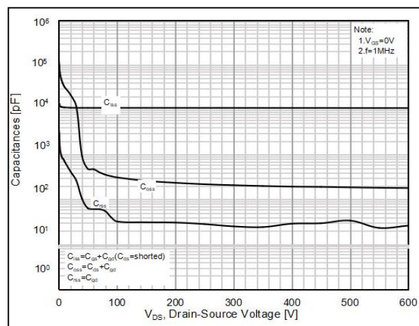
Figure2. Capacitance
