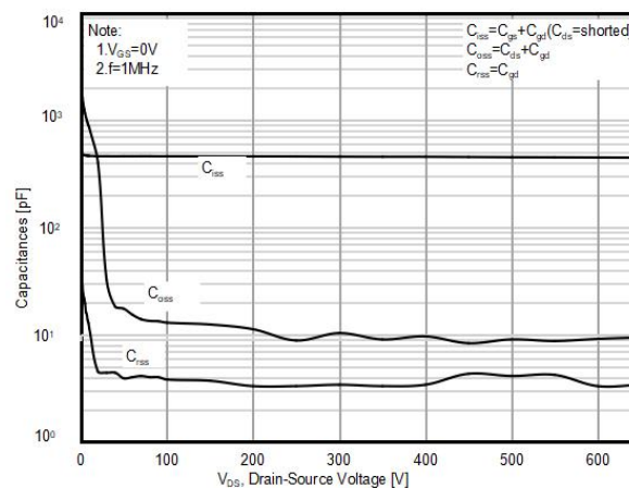
Figure2. Capacitance
