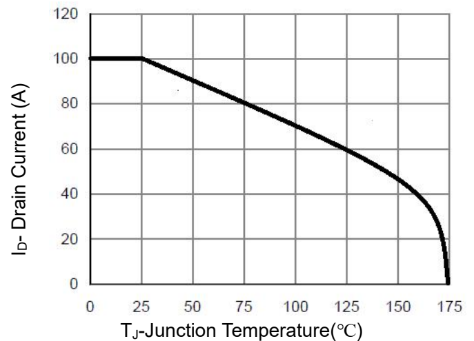
Figure 10 I_{ds} Current De-rating
