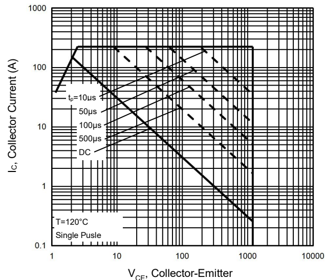
Figure 20 Forward Bias Safe Operating Area
