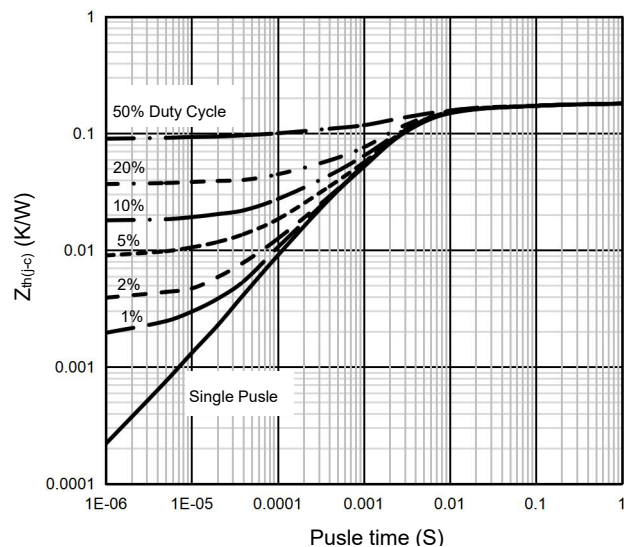
Figure 19 IGBT Transient Thermal Impedance
